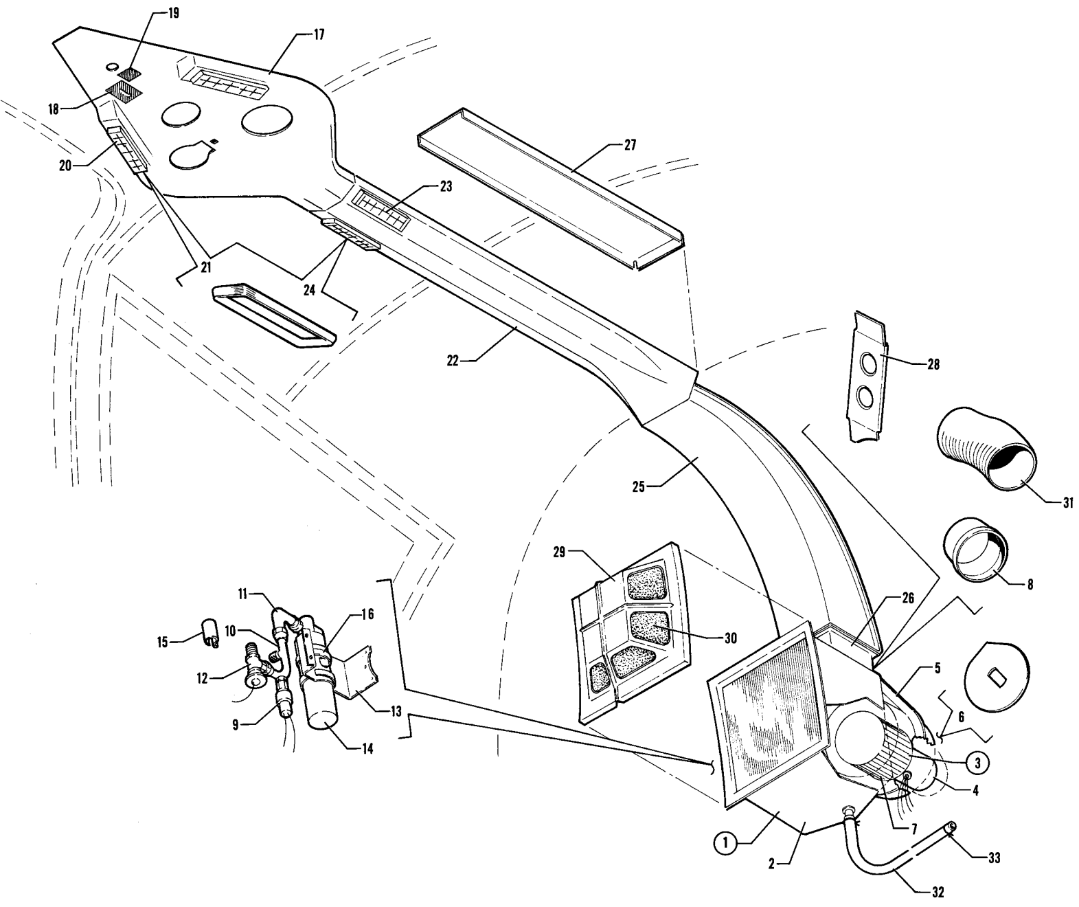
Figure 32B. Air Conditioning Duct and Evaporator Installation
