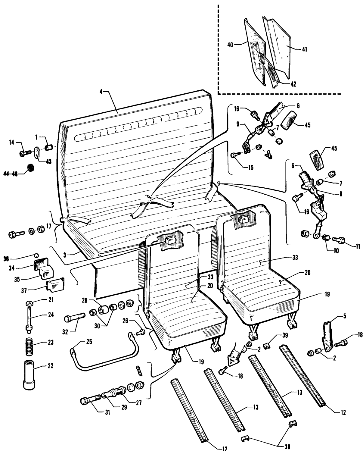
Figure 28. Seats Installation
