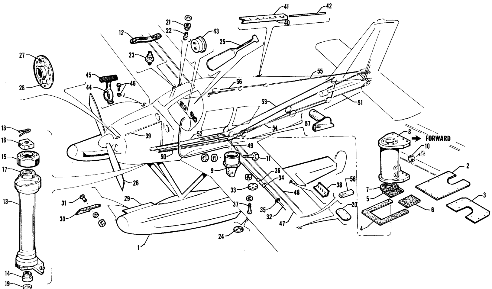
Figure 49. EDO Float Installation
