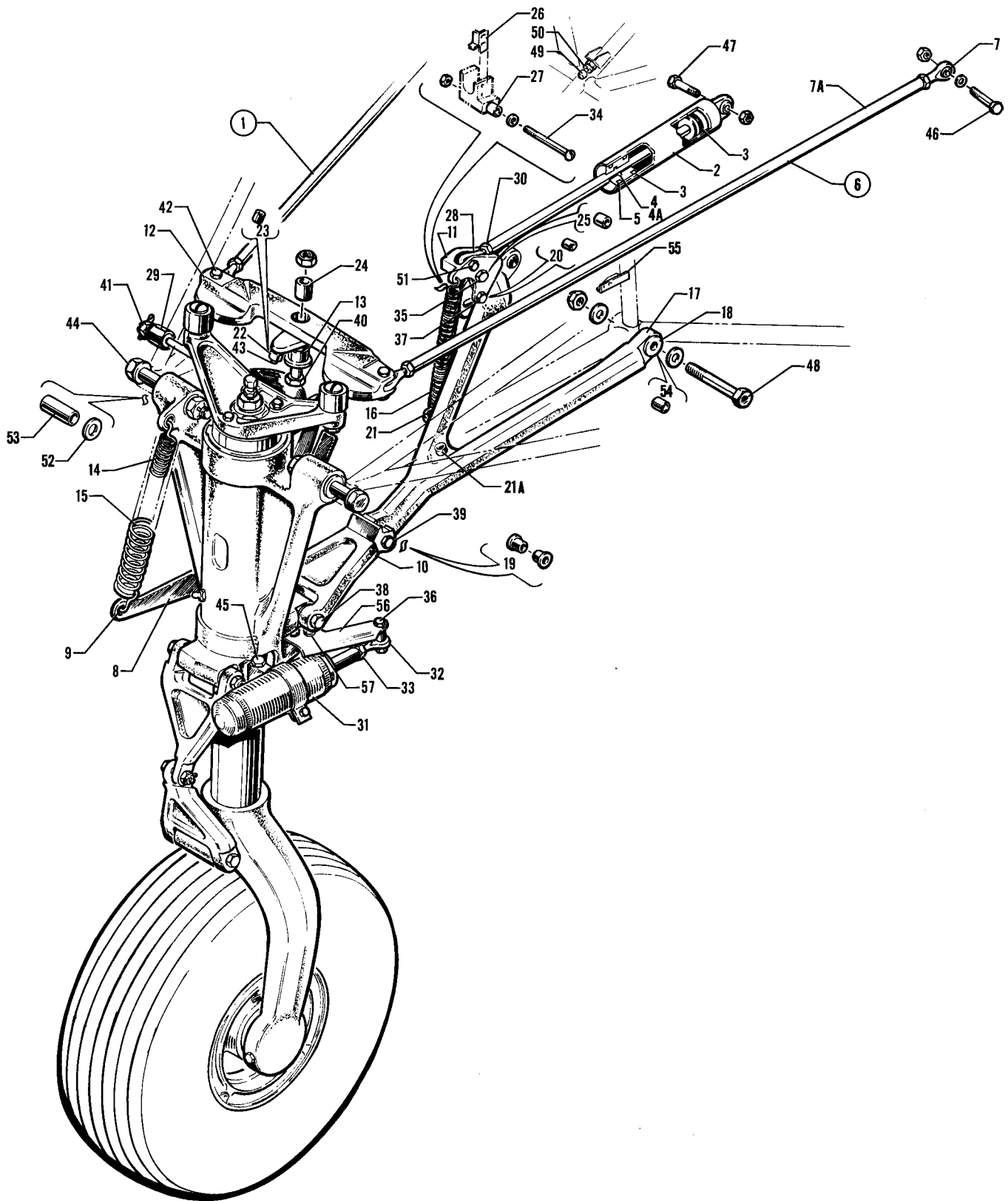
Figure 34. Nose Gear Installation
