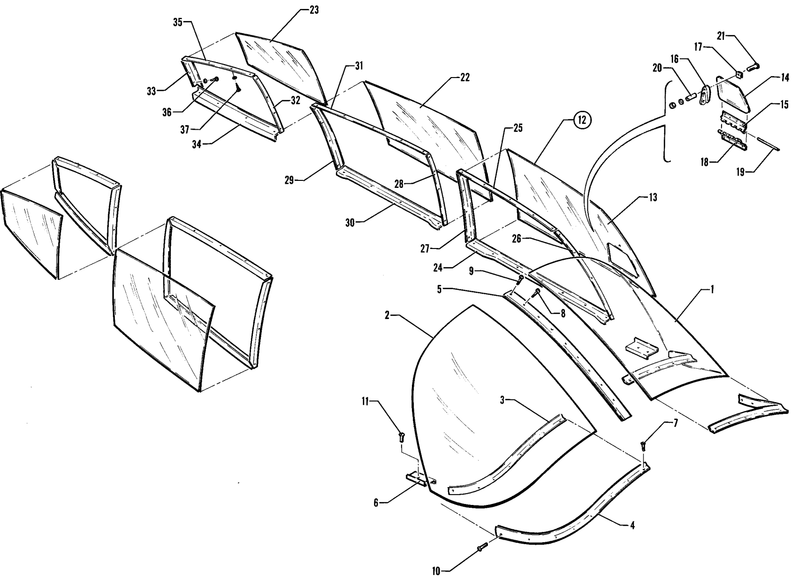
Figure 23. Fuselage Enclosure Installation (PA-28-180 - Serial Nos. 28-4378 and up) (PA-28R-180 - Serial Nos. 28-30005 to 28-30481 inclusive, 28-30483 and up) (PA-28R-200 - Serial Nos. 28-30482, 28-35001 and up)
