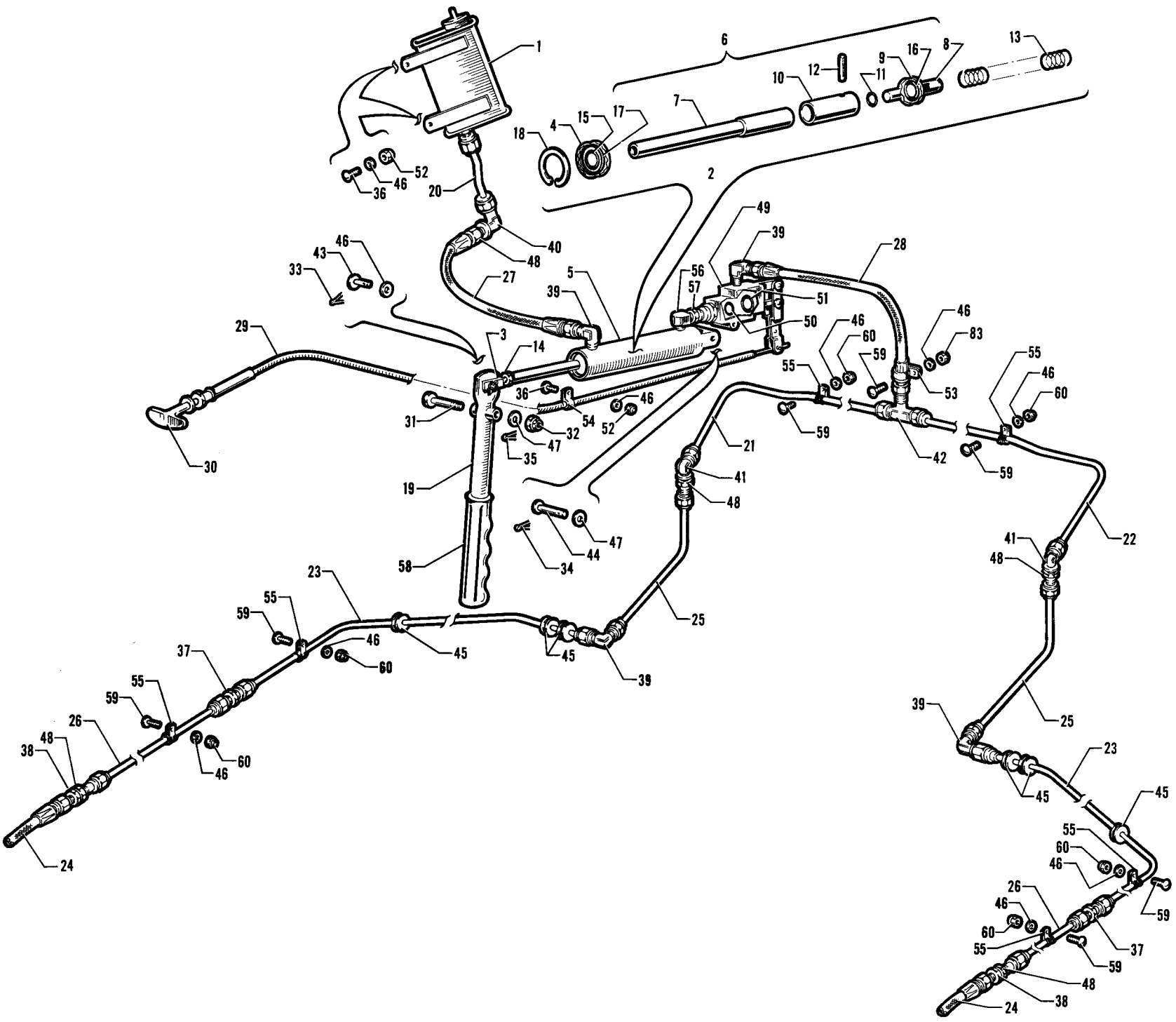
Figure 45. Hand Brake Installation (Serial Nos. 28-1 to 28-250 inclusive)
