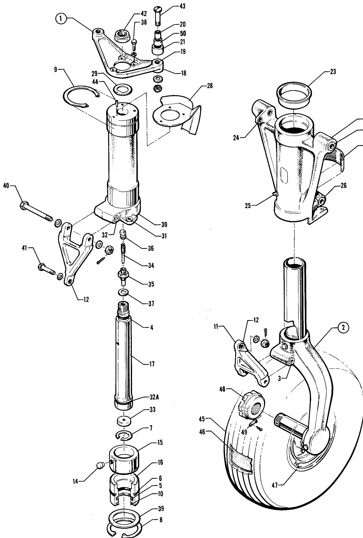
Figure 35. Nose Gear Assembly
