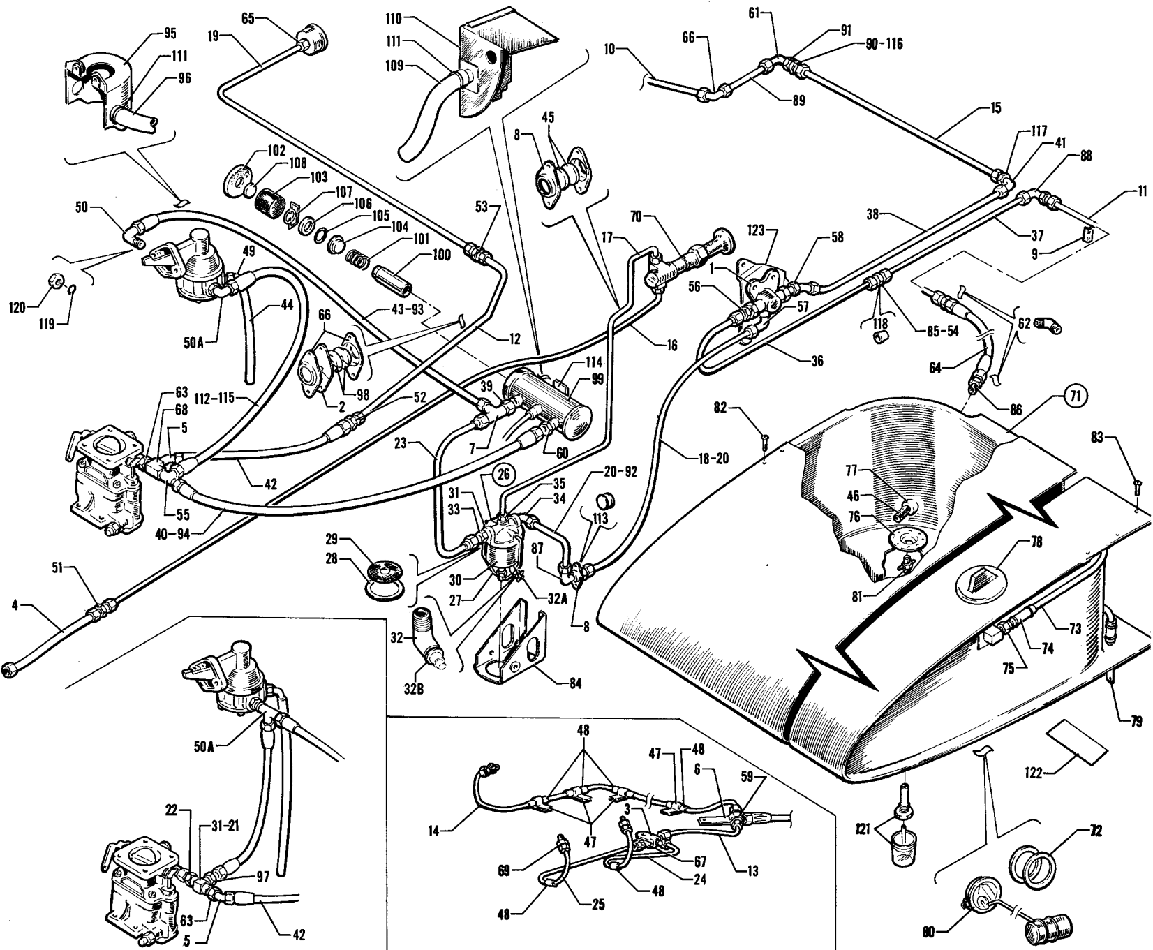
Figure 51. Fuel System Installation
