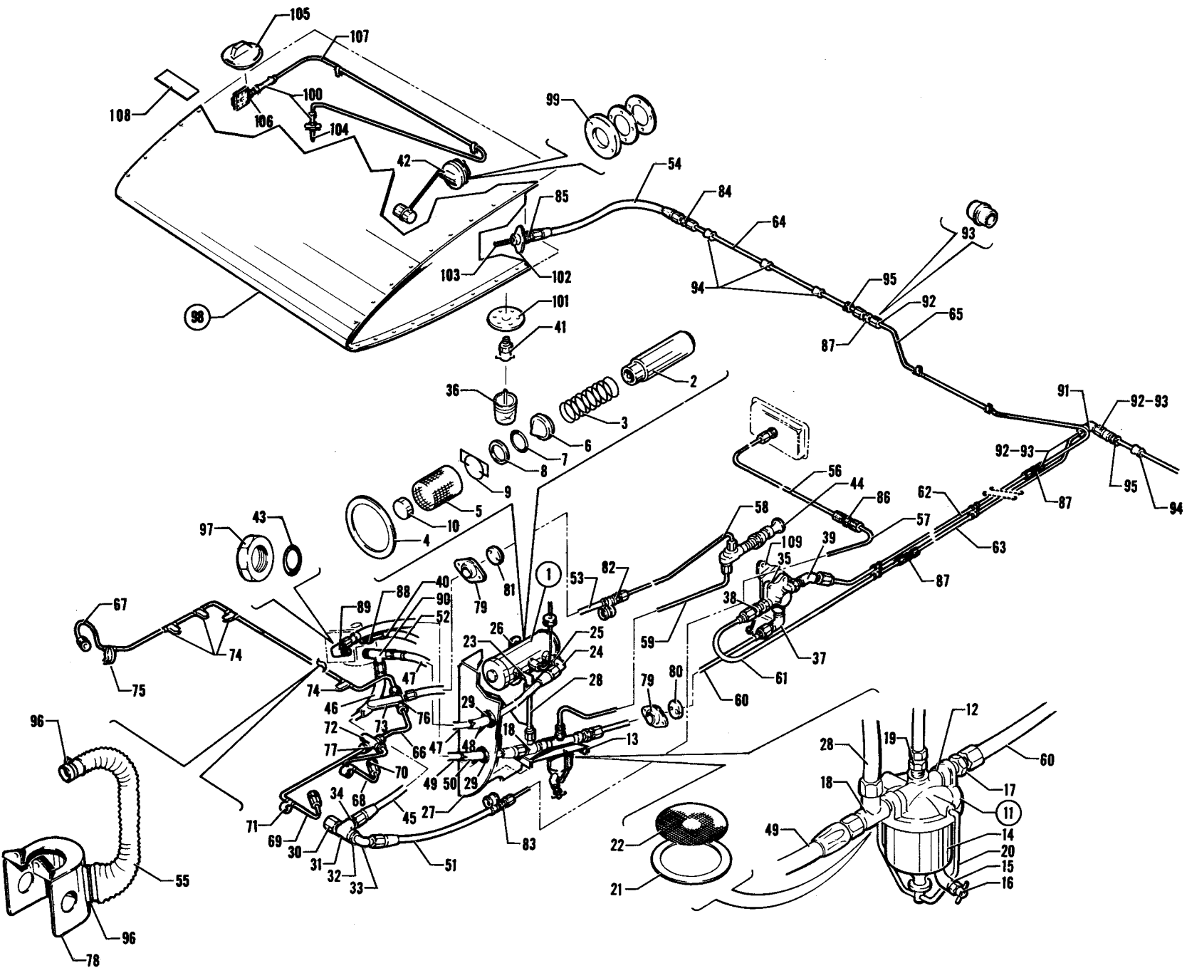
Figure 53. Fuel System Installation (PA-28-150-160-180 - Serial Nos. 28-1761 and up)
