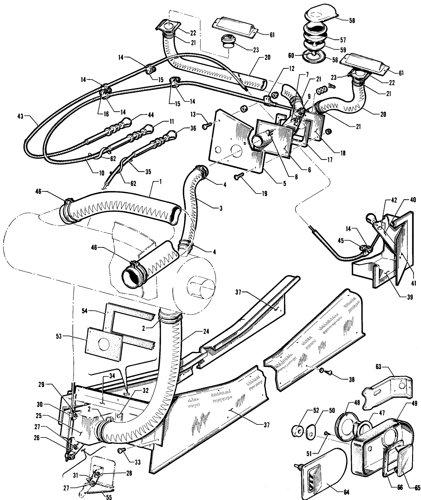
Figure 30. Cabin Heat, Defroster and Fresh Air System (PA-28-140 - Serial Nos. 28-20002 to 28-24999 inclusive) (PA-28-150-160-180 - Serial Nos. 28-1 to 28-1760 inclusive)
