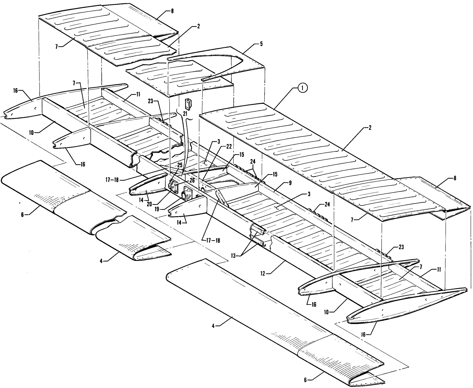
Figure 50A. Stabilator Assembly (Serial Nos. 28-7235001 and up)
