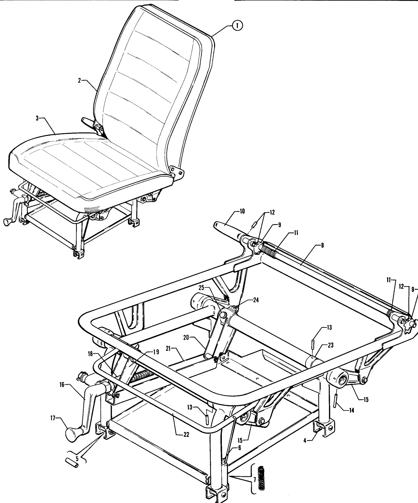
Figure 28B. Vertically Adjustable Front Seat Assembly
