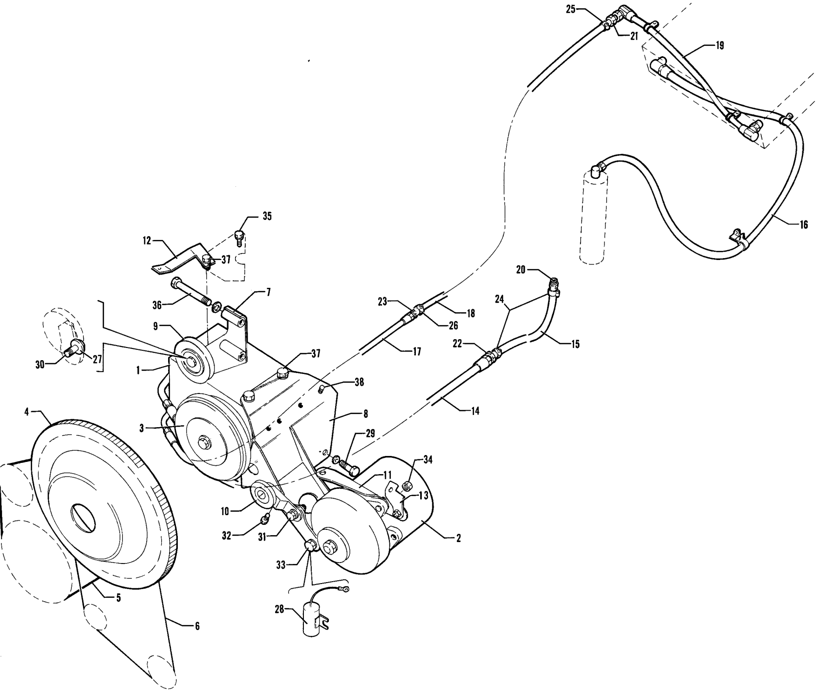
Figure 32A. Air Conditioning Compressor, Refrigerant Lines and Alternator Installation (PA-28-140 - Serial Nos. 28-7125472 and up) (PA-28-180 - Serial Nos. 28-7205092 and up) (PA-28R-200 - Serial Nos. 28-7235001 and up)
