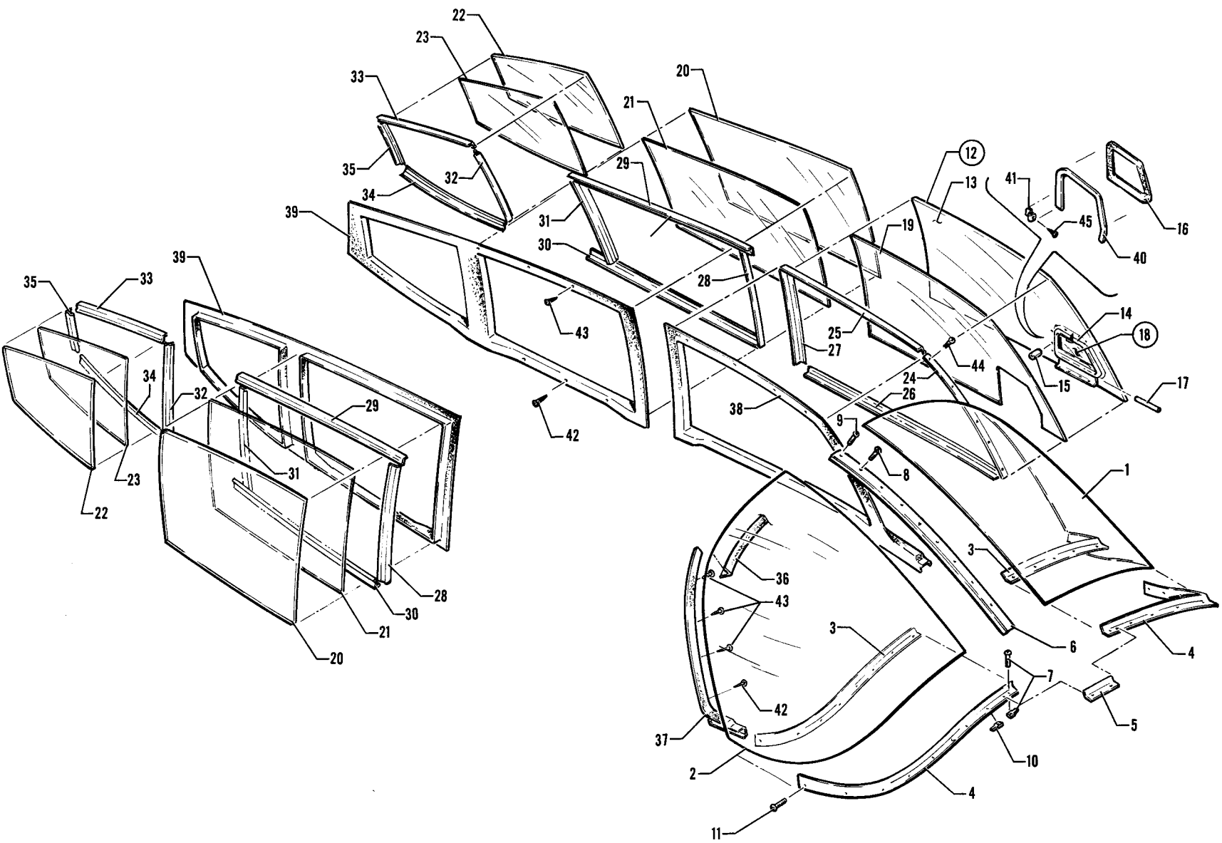
Figure 22A. Fuselage Enclosure Installation (PA-28-235 - Serial Nos. 28-11040 and up)
