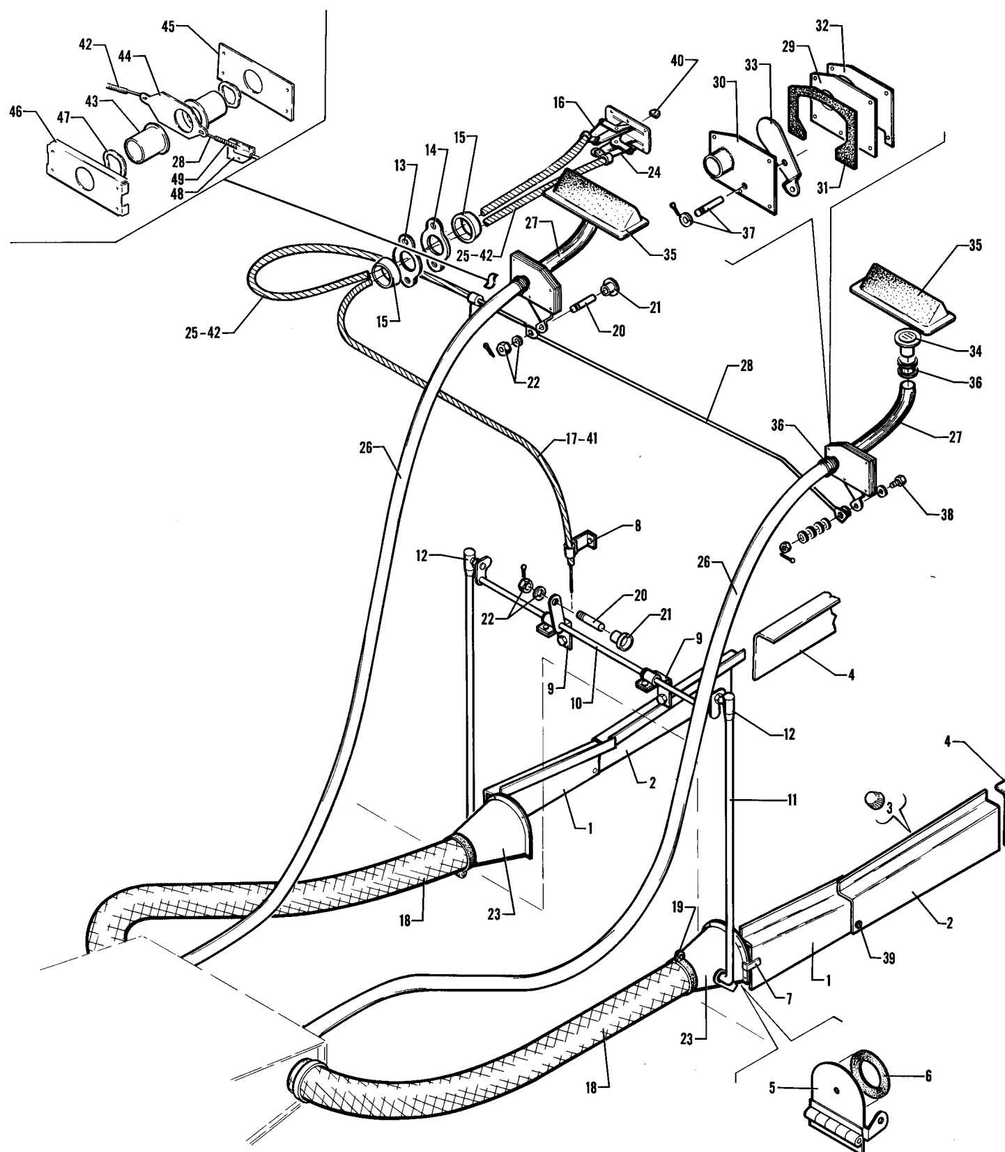
Figure 32. Cabin Heat and Defroster Installation
