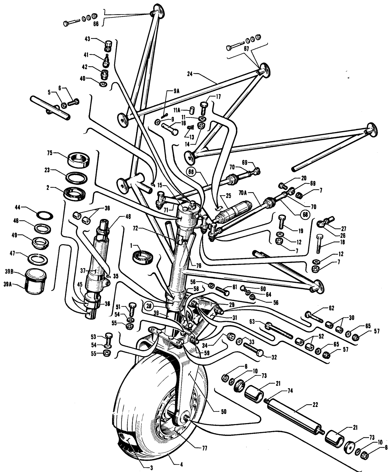
Figure 33. Nose Gear Installation
