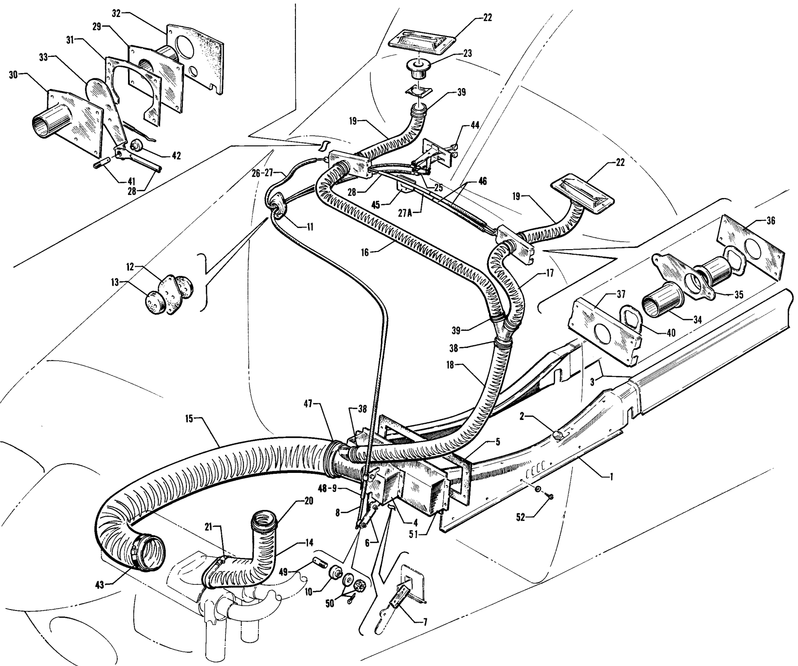
Figure 31A. Cabin Heat and Defroster Installation (PA-28-180 - Serial Nos. 28-4378 and up) (PA-28-235 - Serial Nos. 28-11040 and up)
