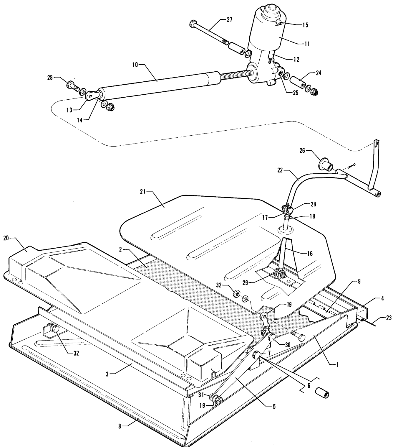
Figure 32C. Air Conditioning Condenser Installation (PA-28-140 - Serial Nos. 28-7125472 and up) (PA-28-180 - Serial Nos. 28-7205092 and up) (PA-28R-200 - Serial Nos. 28-7235001 and up)
