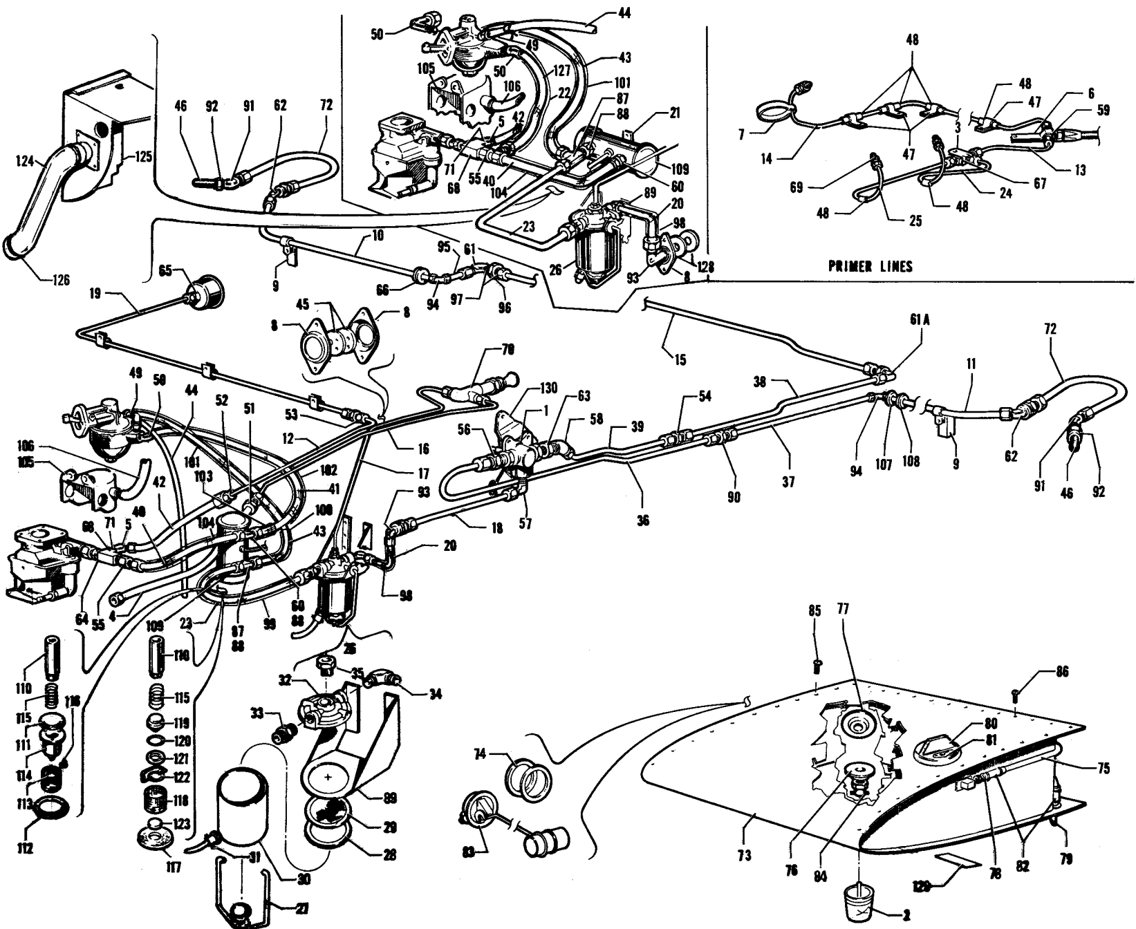
Figure 52. Fuel System Installation (PA-28-150-160-180 - Serial Nos. 28-1 to 28-1760 inclusive)
