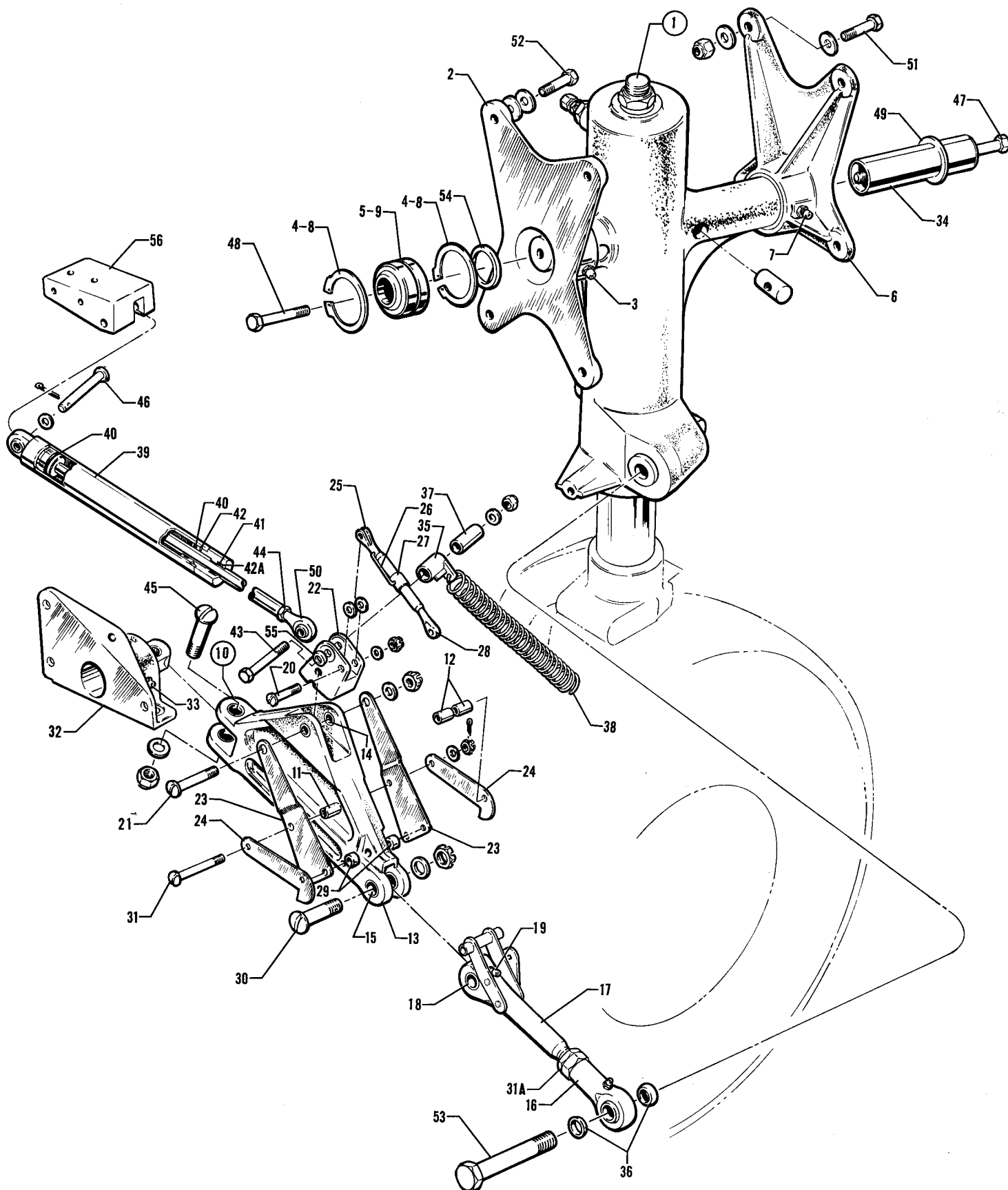
Figure 38. Main Gear Installation
