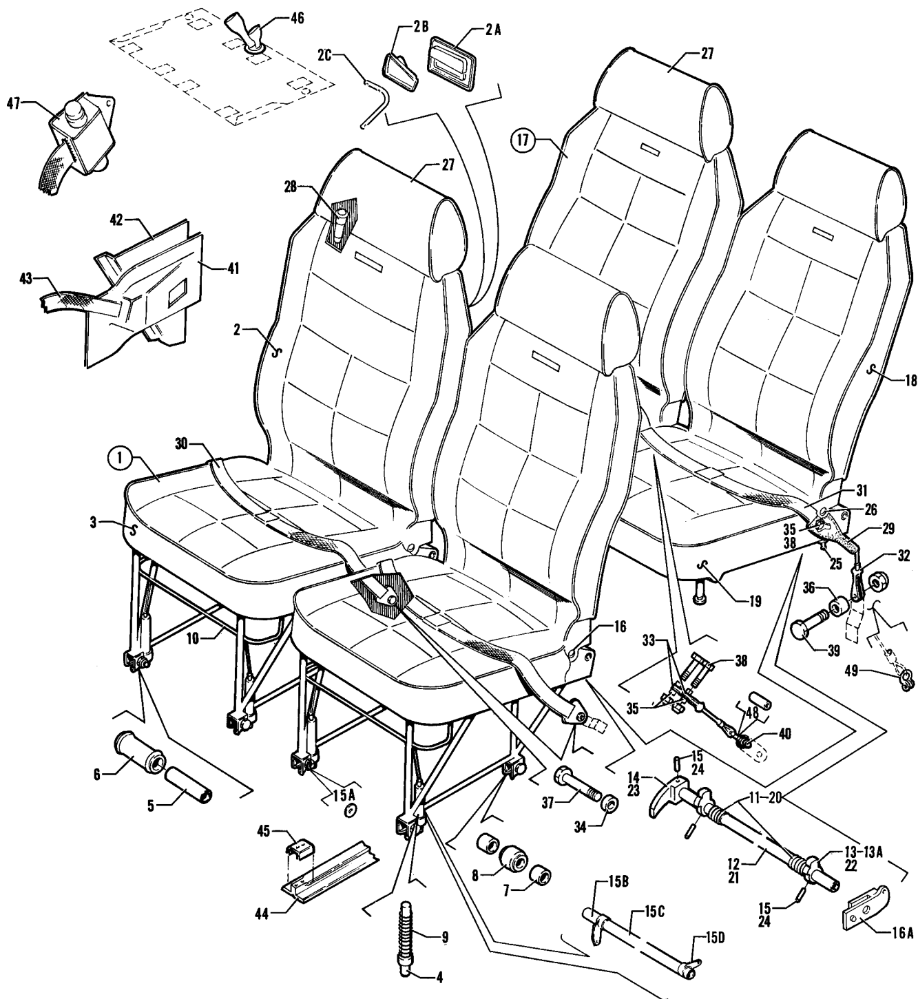
Figure 28A. Seats Installation (PA-28-140 - Serial Nos. 28-7125001 and up) (PA-28-180 - Serial Nos. 28-7105001 and up) (PA-28R-180 - Serial Nos. 28-7130001 and up) (PA-28R-200 - Serial Nos. 28-7135001 and up) (PA-28-235 - Serial Nos. 28-7110001 and up)
