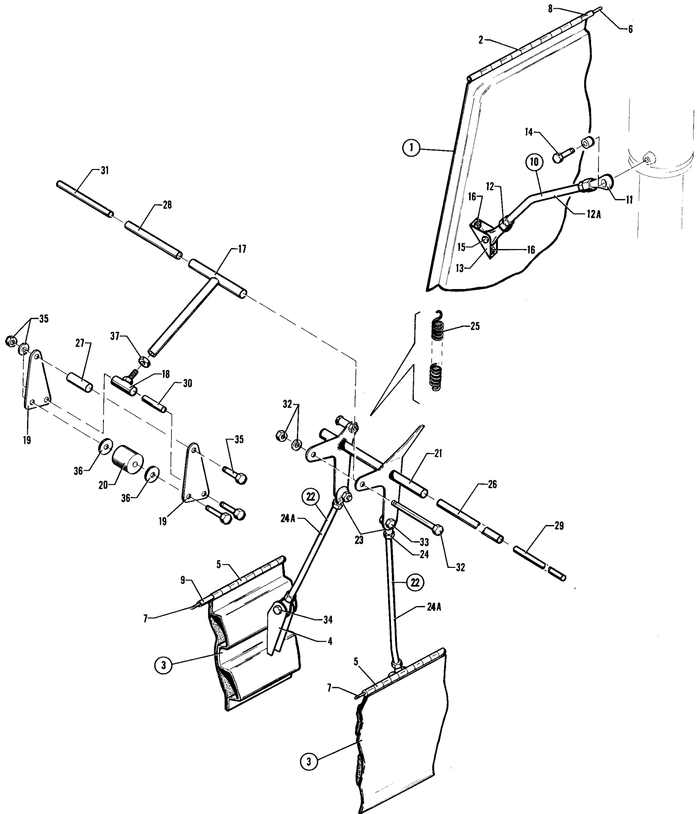
Figure 42. Landing Gear Door Installation
