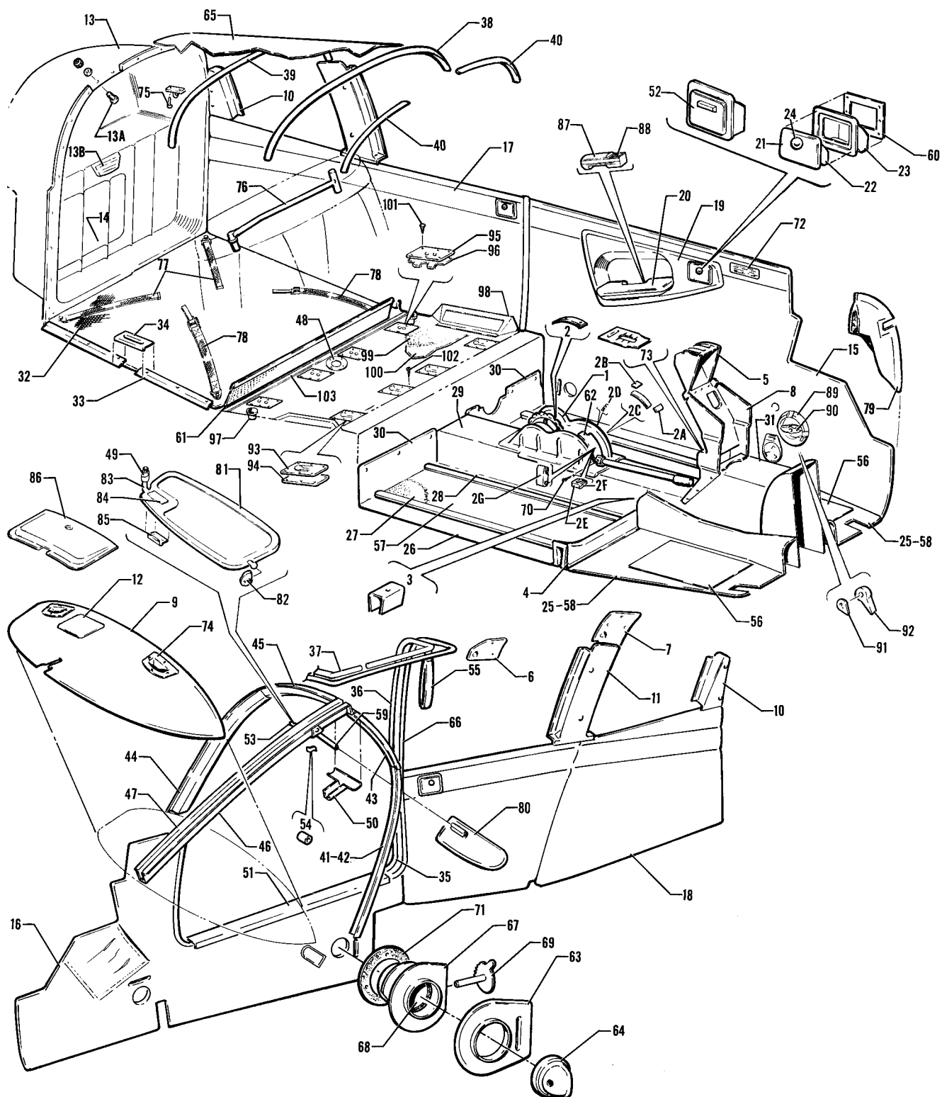
Figure 27. Cockpit Finishing Installation (PA-28-180 - Serial Nos. 28-4378 and up) (PA-28R-180 - Serial Nos. 28-30005 to 28-30481 inclusive, 28-30483 and up) (PA-28R-200 - Serial Nos. 28-30482, 28-35001 and up)
